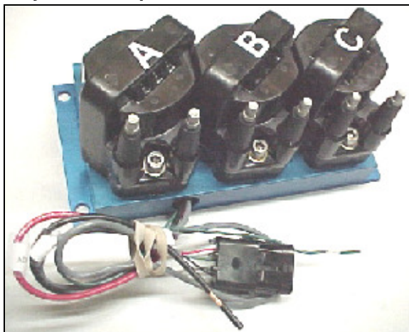
6 Cylinder coil pack
