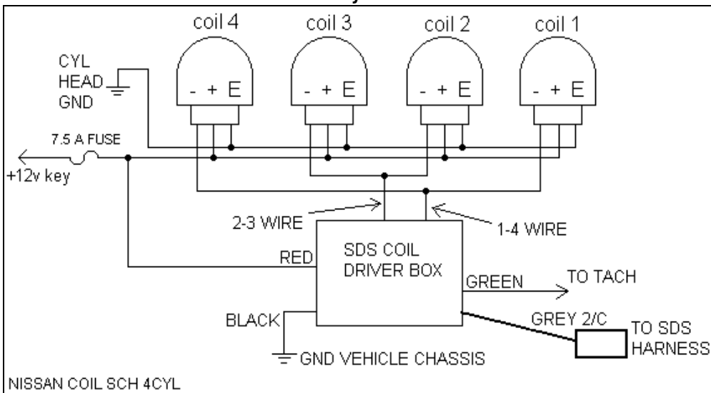
NISSAN COIL SCH 4CYL
