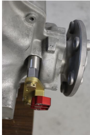
Standoff detail
