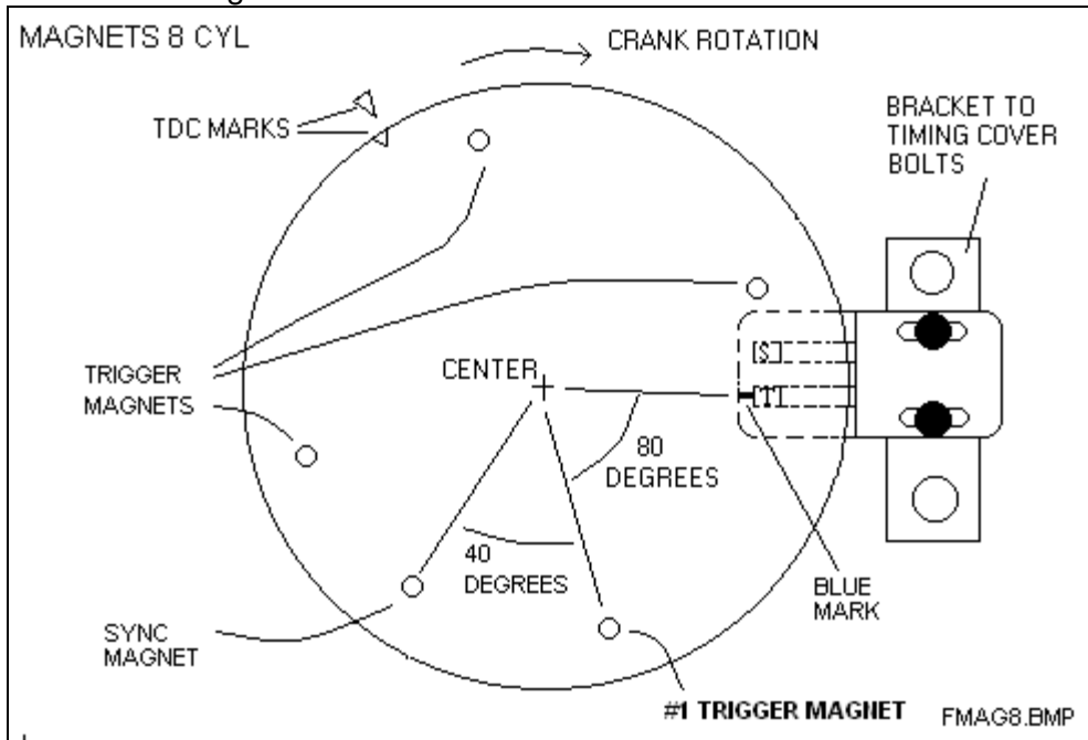
End view of magnet locations relative to the sensor.
